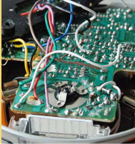
Shoddy workmanship, which compromises the durability of a system, can usually be recognised at sight. Photo: ISE
